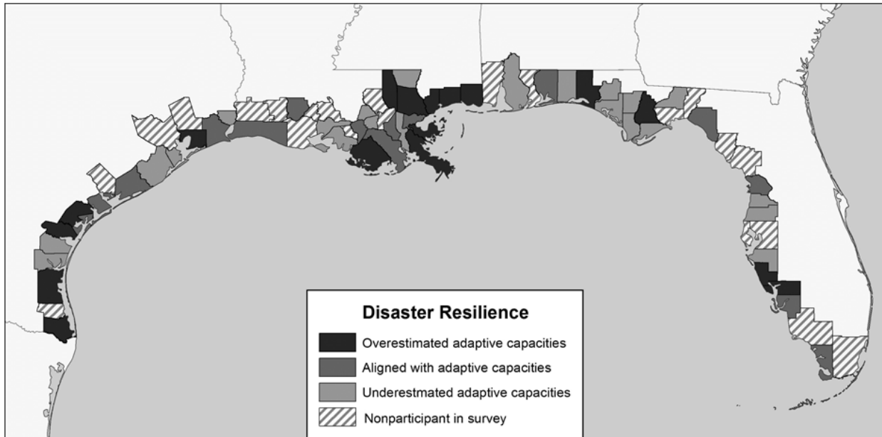
Figure 7.3: Map of the Alignment of Resilience Perceptions and Realities
